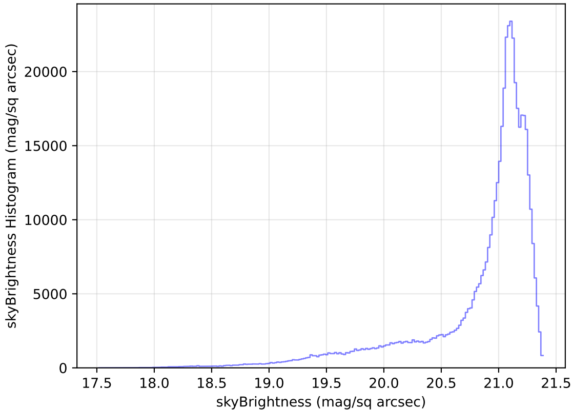
weather_cloudso18v3.4_10yrs WFD r band: skyBrightness Histogram
