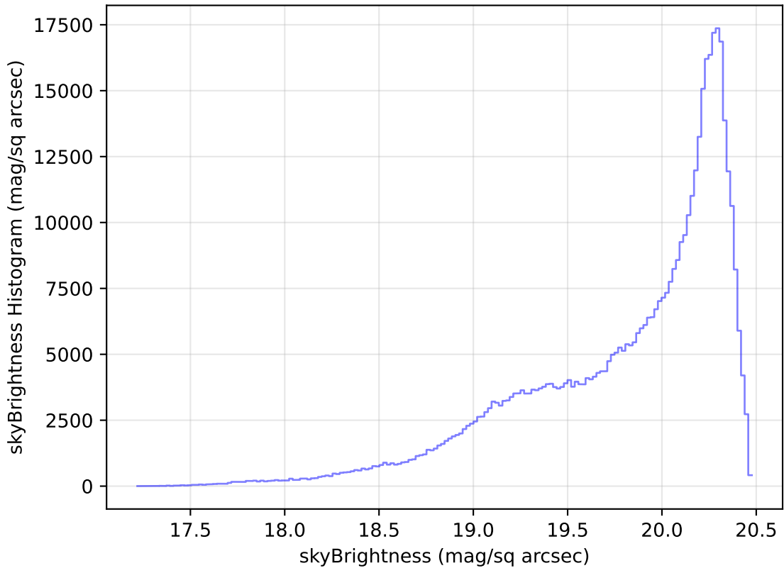
weather_cloudso18v3.4_10yrs WFD i band: skyBrightness Histogram
