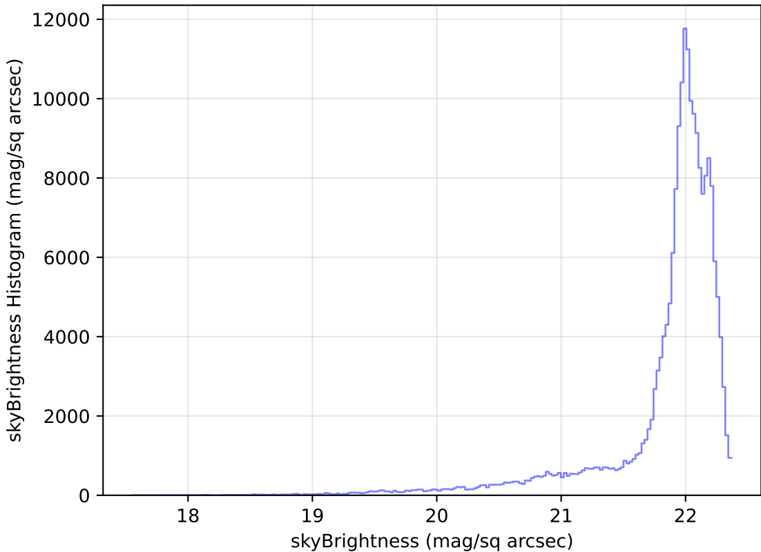
weather_cloudso18v3.4_10yrs WFD g band: skyBrightness Histogram
