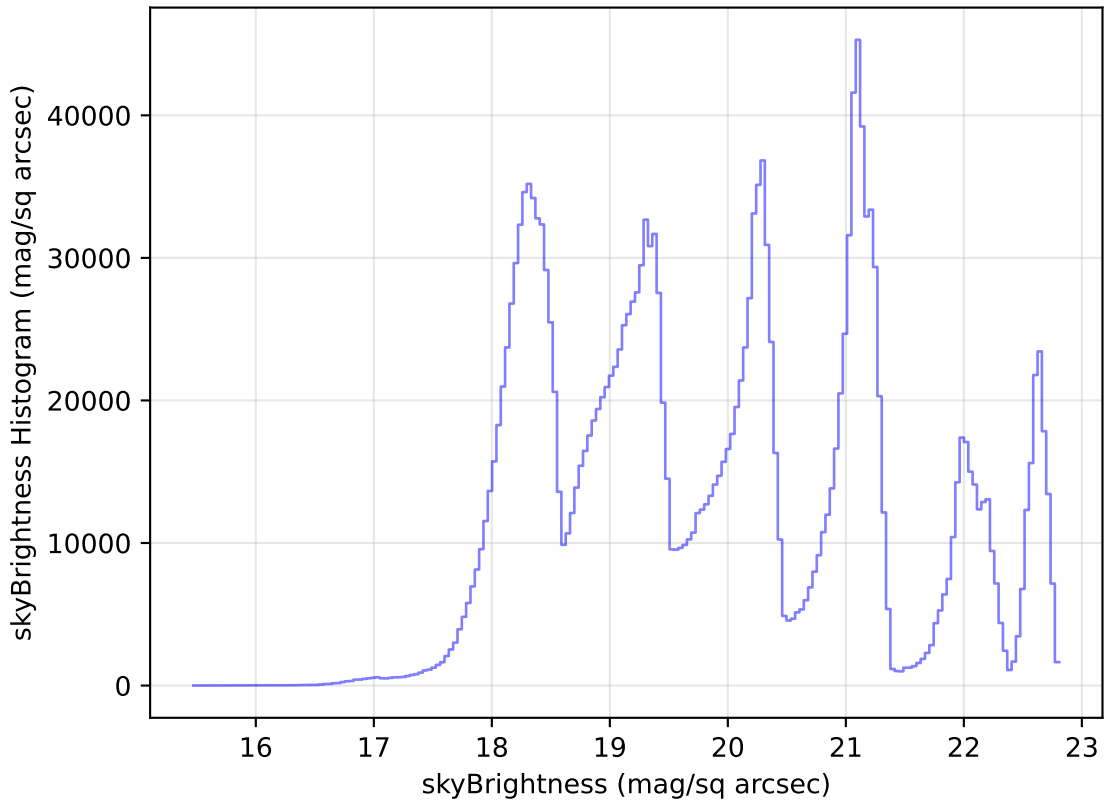
weather_cloudso18v3.4_10yrs WFD all bands: skyBrightness Histogram
