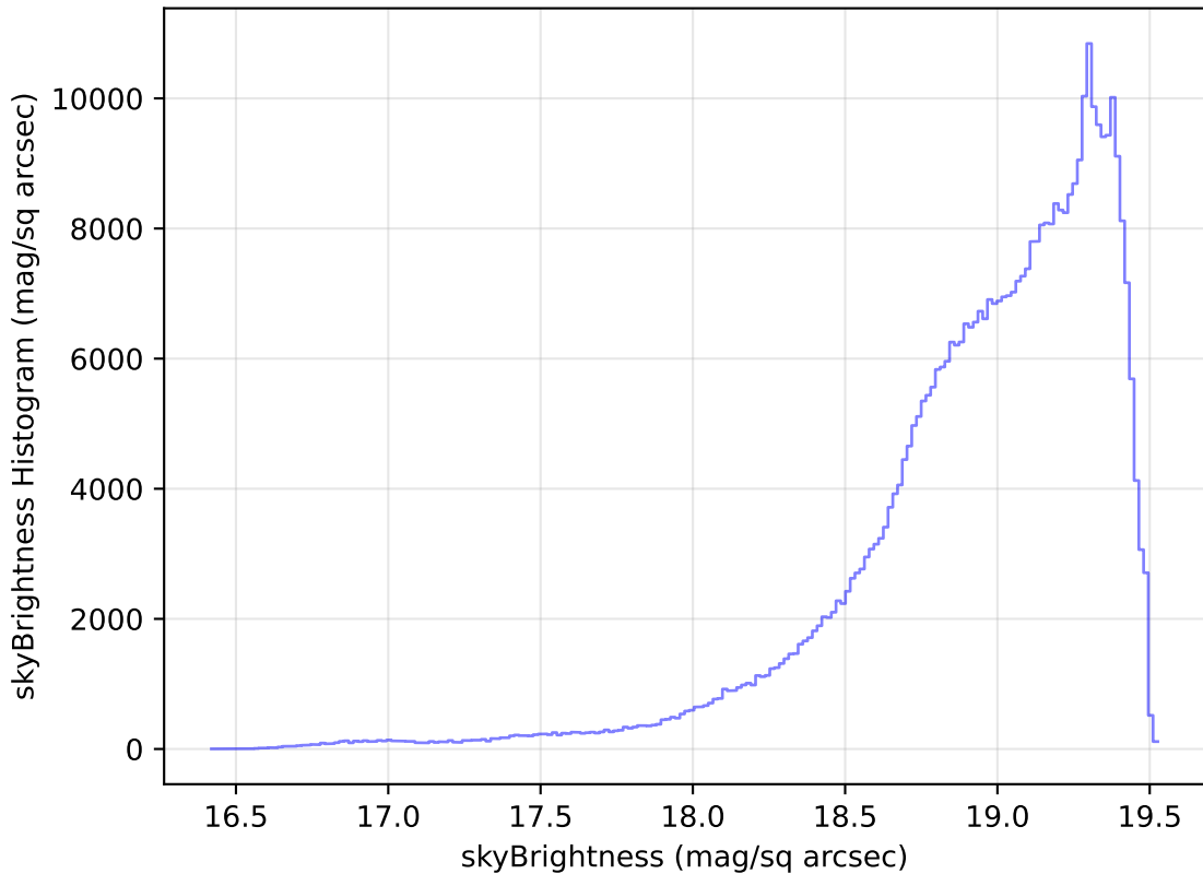
weather_cloudso18v3.4_10yrs All sky z band: skyBrightness Histogram
