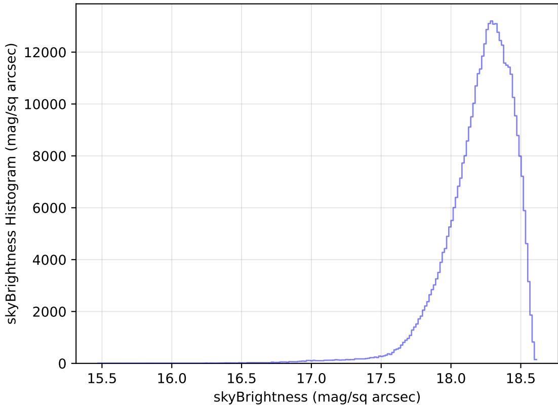
weather_cloudso18v3.4_10yrs All sky y band: skyBrightness Histogram
