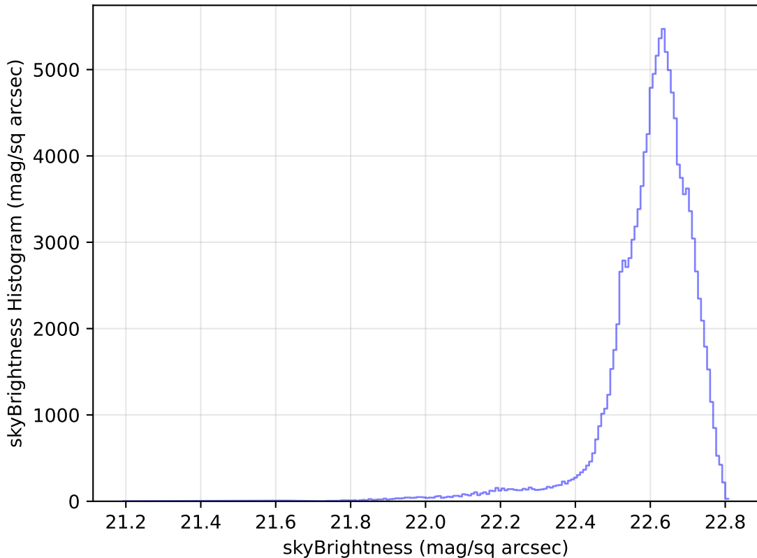
weather_cloudso18v3.4_10yrs All sky u band: skyBrightness Histogram
