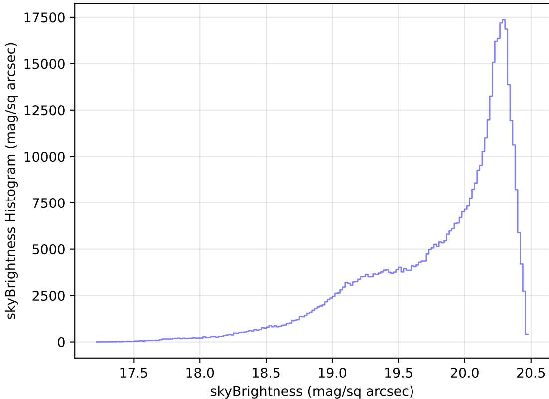
weather_cloudso18v3.4_10yrs All sky i band: skyBrightness Histogram
