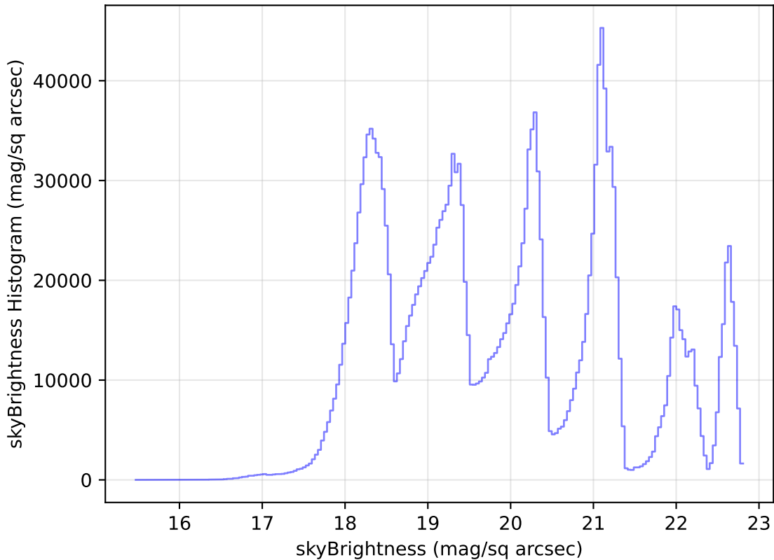
weather_cloudso18v3.4_10yrs All sky all bands: skyBrightness Histogram
