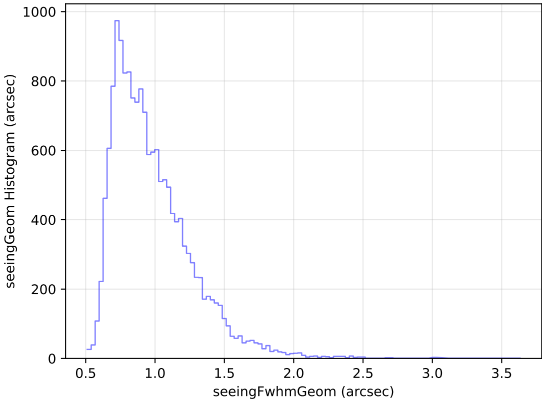
weather_cloudso18v3.4_10yrs Yr 1 u band: seeingGeom Histogram
