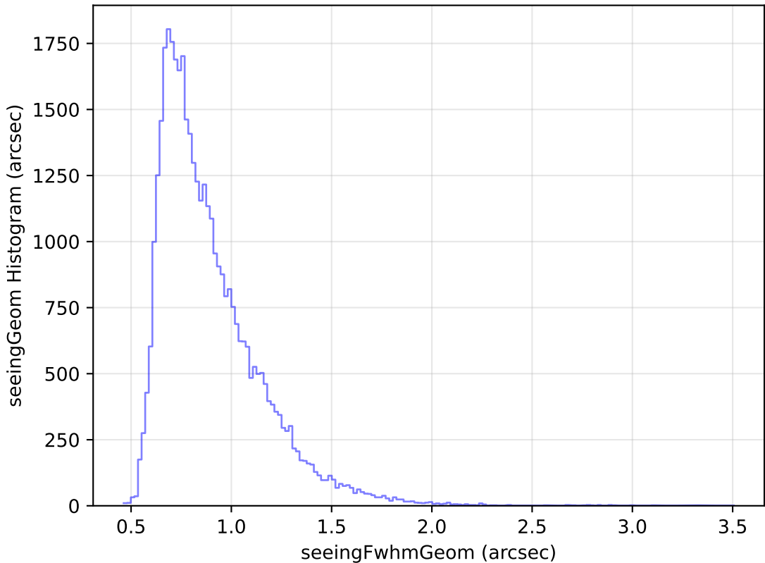
weather_cloudso18v3.4_10yrs Yr 1 r band: seeingGeom Histogram
