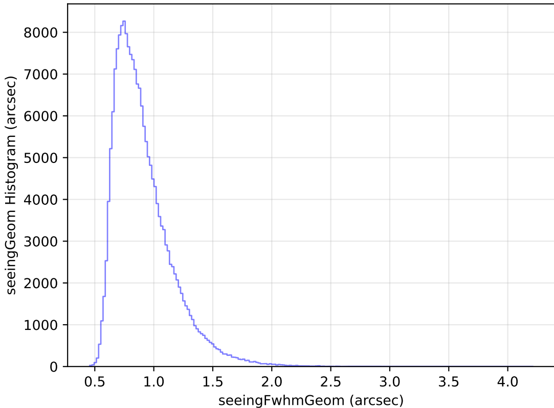
weather_cloudso18v3.4_10yrs Yr 1 all bands: seeingGeom Histogram
