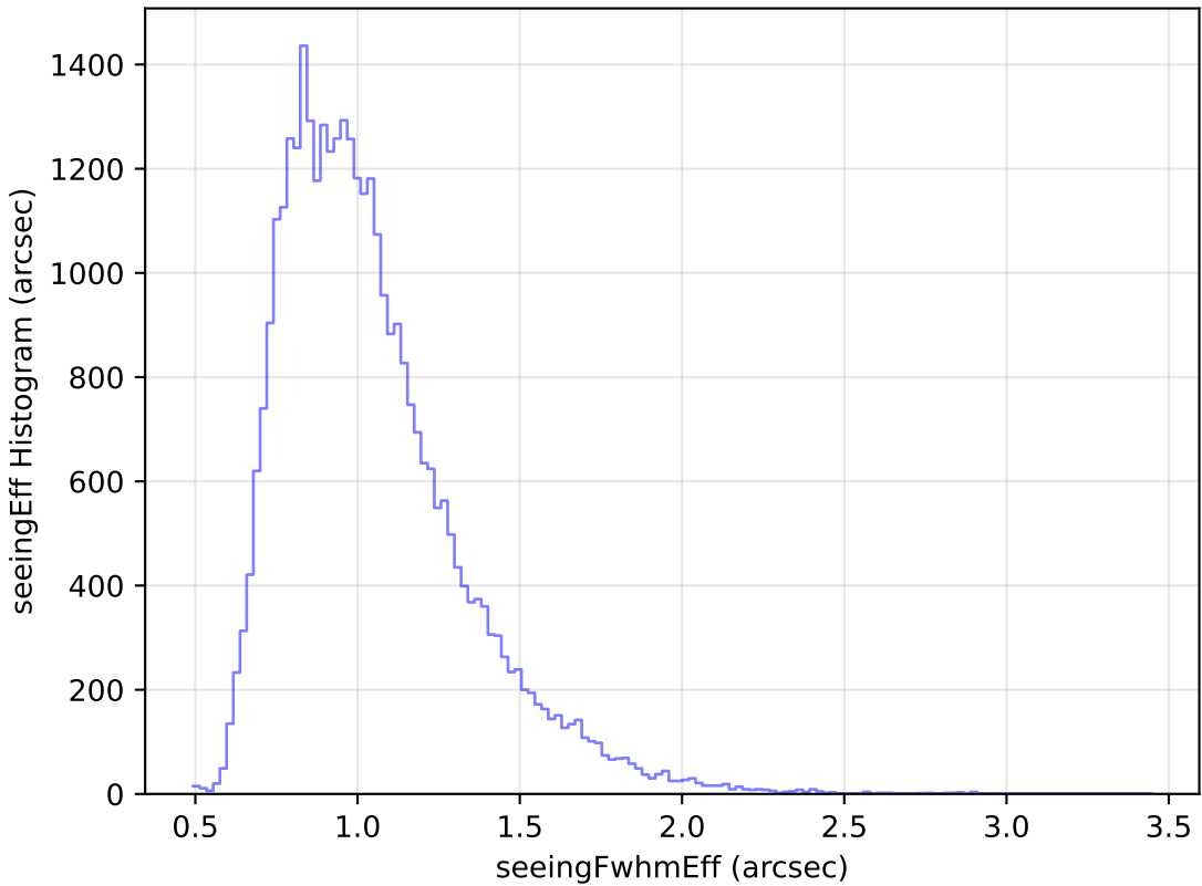
weather_cloudso18v3.4_10yrs Yr 1 z band: seeingEff Histogram
