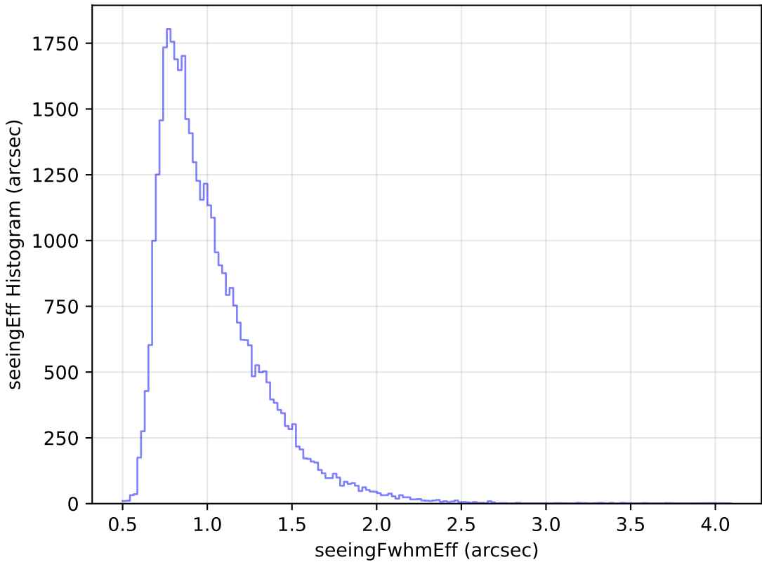
weather_cloudso18v3.4_10yrs Yr 1 r band: seeingEff Histogram
