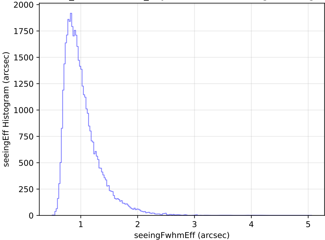
weather_cloudso18v3.4_10yrs Yr 1 i band: seeingEff Histogram
