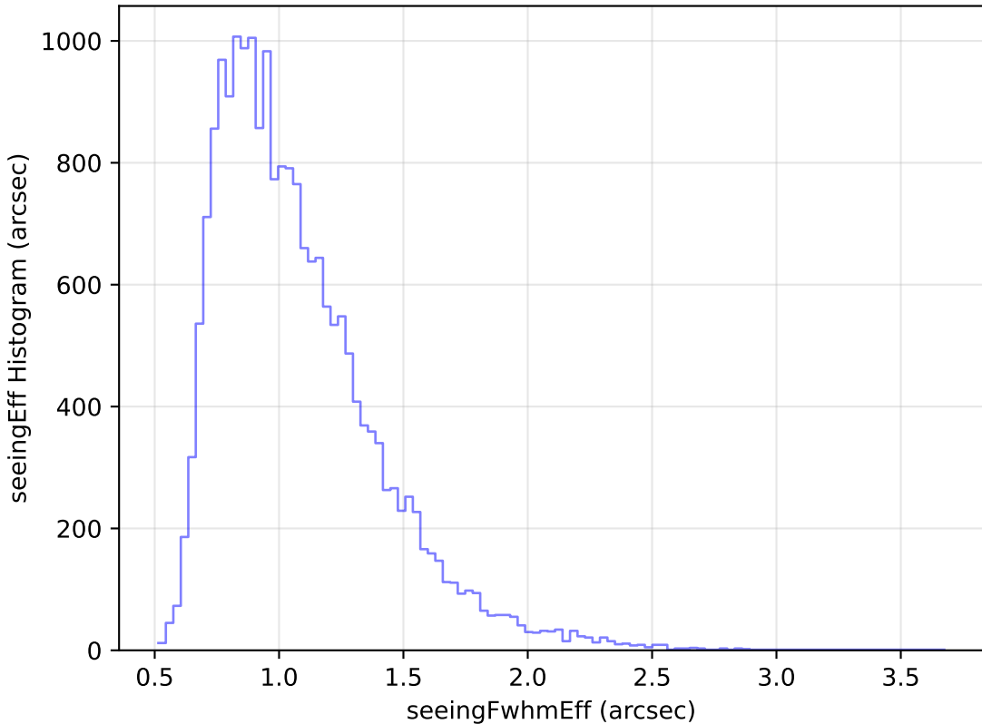
weather_cloudso18v3.4_10yrs Yr 1 g band: seeingEff Histogram
