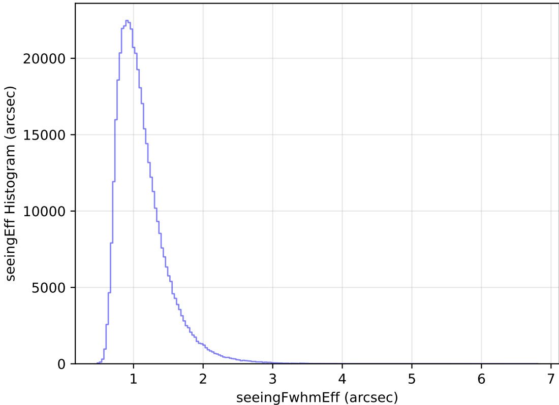
weather_cloudso18v3.4_10yrs WFD z band: seeingEff Histogram
