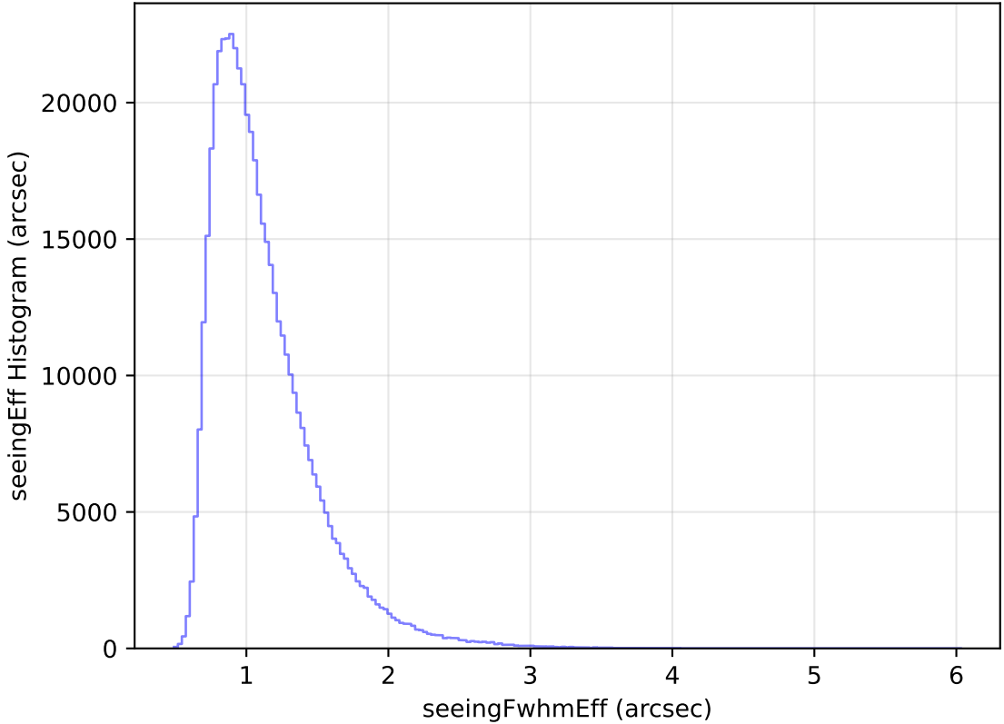
weather_cloudso18v3.4_10yrs WFD i band: seeingEff Histogram
