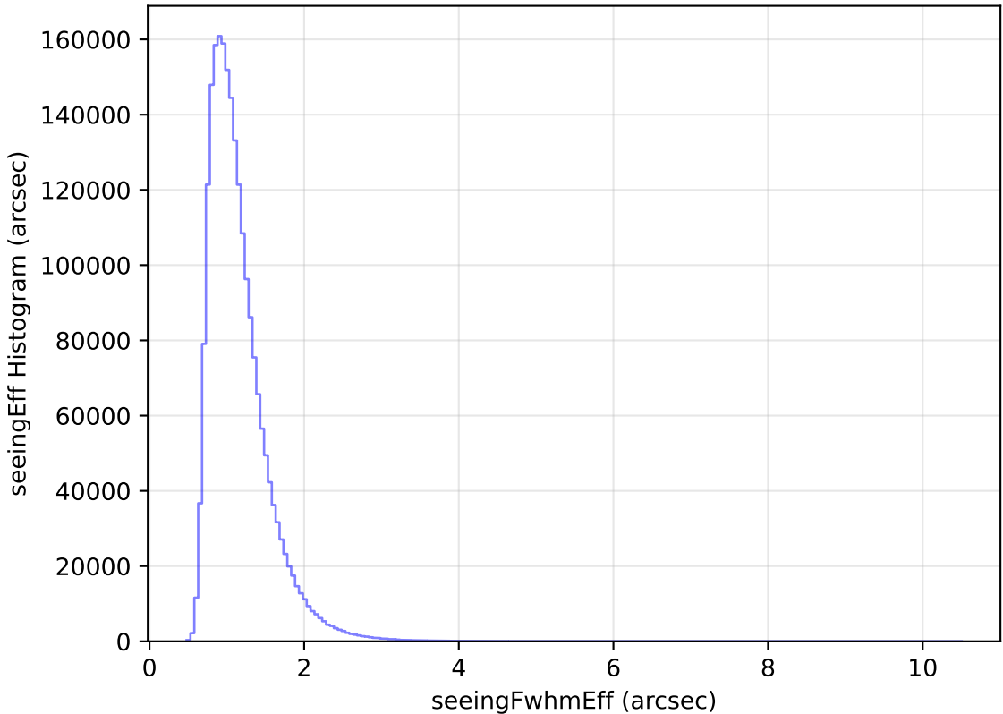
weather_cloudso18v3.4_10yrs WFD all bands: seeingEff Histogram
