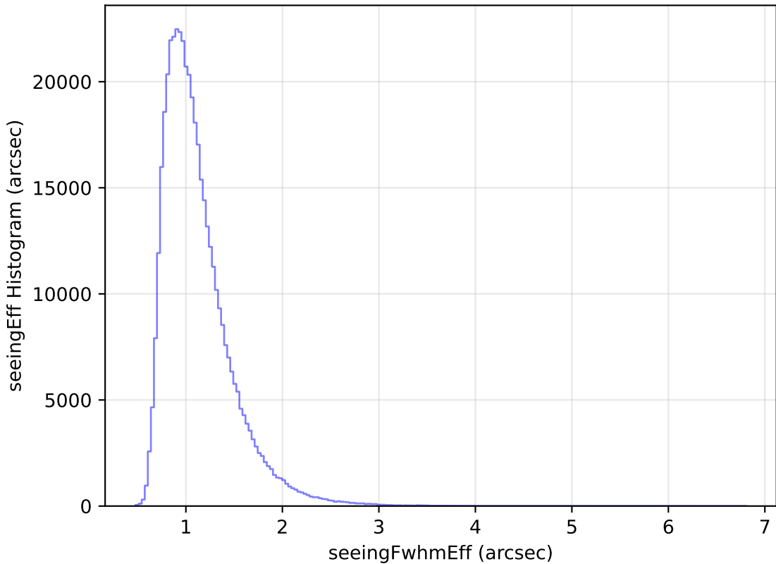
weather_cloudso18v3.4_10yrs All sky z band: seeingEff Histogram
