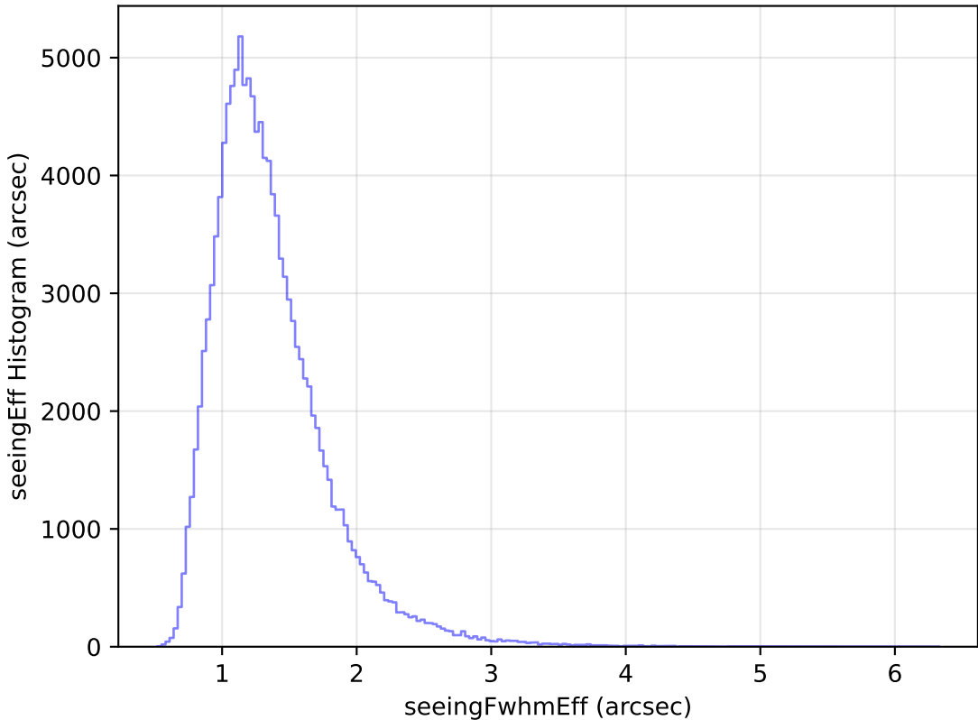
weather_cloudso18v3.4_10yrs All sky u band: seeingEff Histogram
