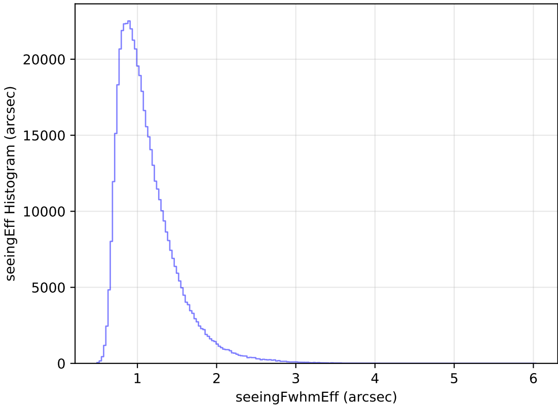
weather_cloudso18v3.4_10yrs All sky i band: seeingEff Histogram
