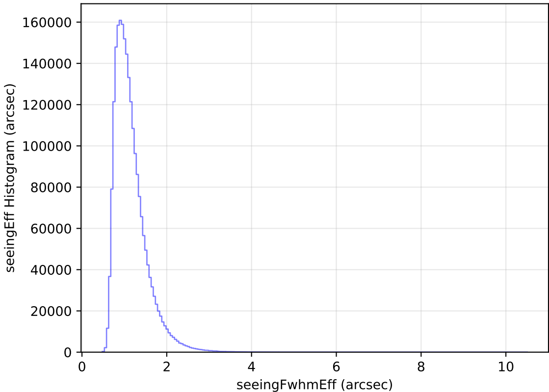
weather_cloudso18v3.4_10yrs All sky all bands: seeingEff Histogram
