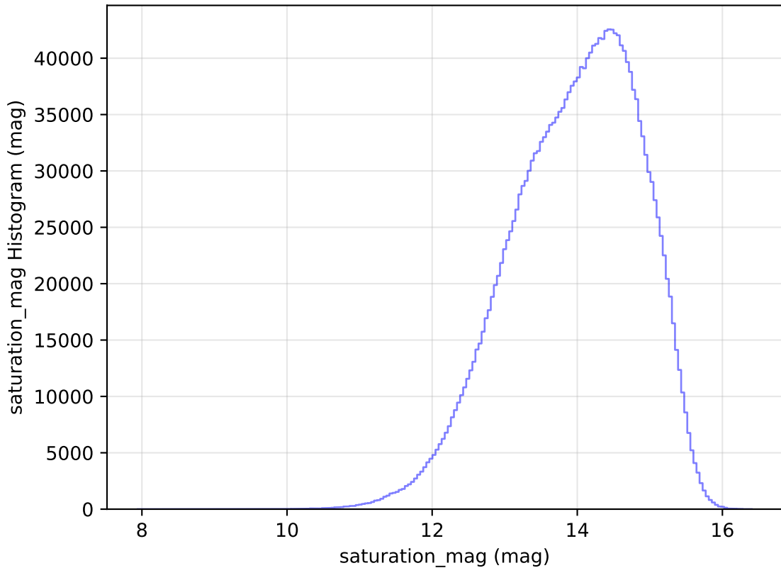
weather_cloudso18v3.4_10yrs WFD all bands: saturation_mag Histogram
