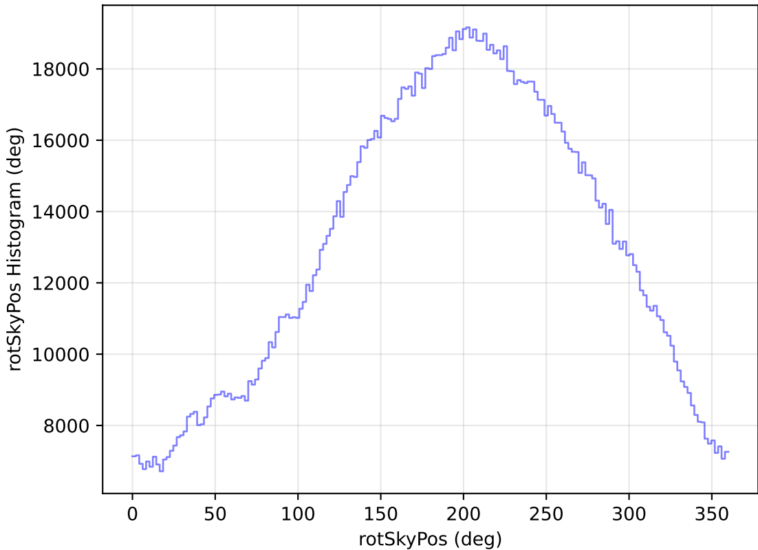
weather_cloudso18v3.4_10yrs WFD all bands: rotSkyPos Histogram
