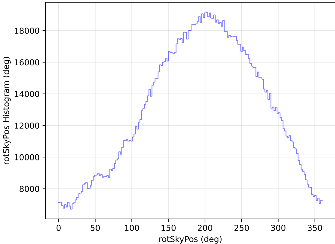
weather_cloudso18v3.4_10yrs All sky all bands: rotSkyPos Histogram
