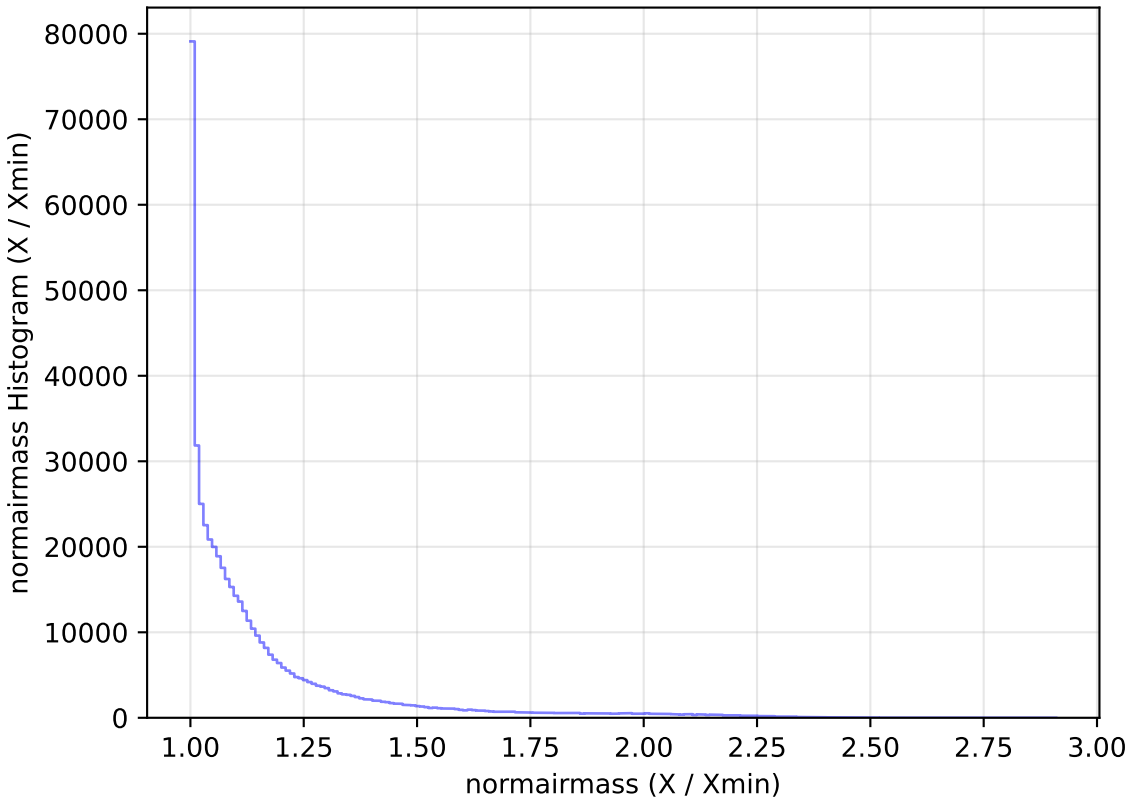
weather_cloudso18v3.4_10yrs WFD r band: normairmass Histogram
