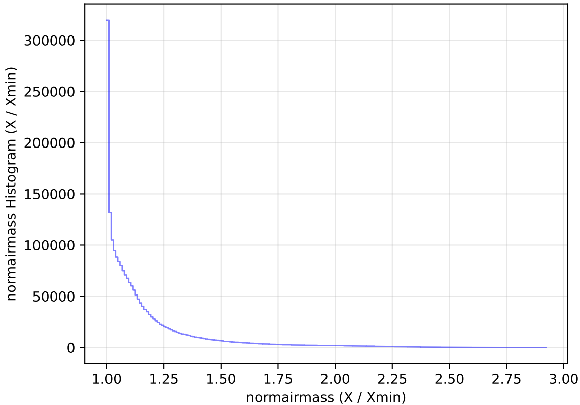
weather_cloudso18v3.4_10yrs WFD all bands: normairmass Histogram
