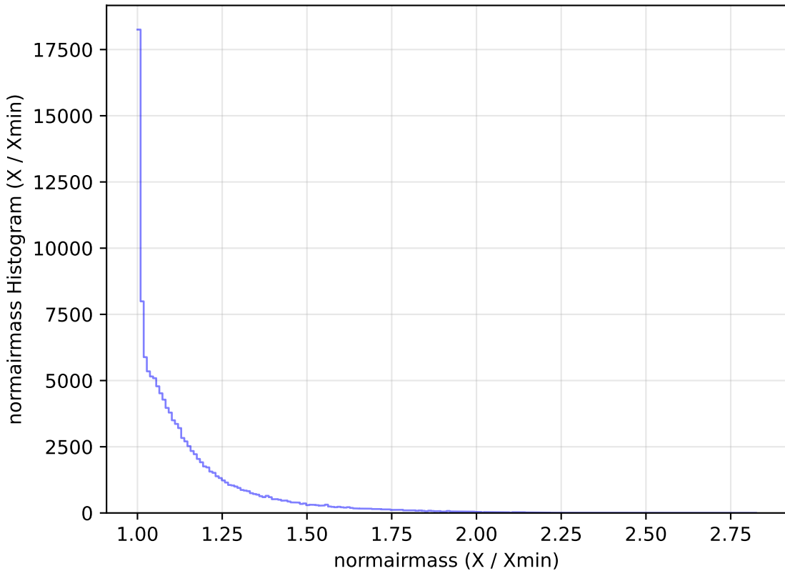
weather_cloudso18v3.4_10yrs All sky u band: normairmass Histogram
