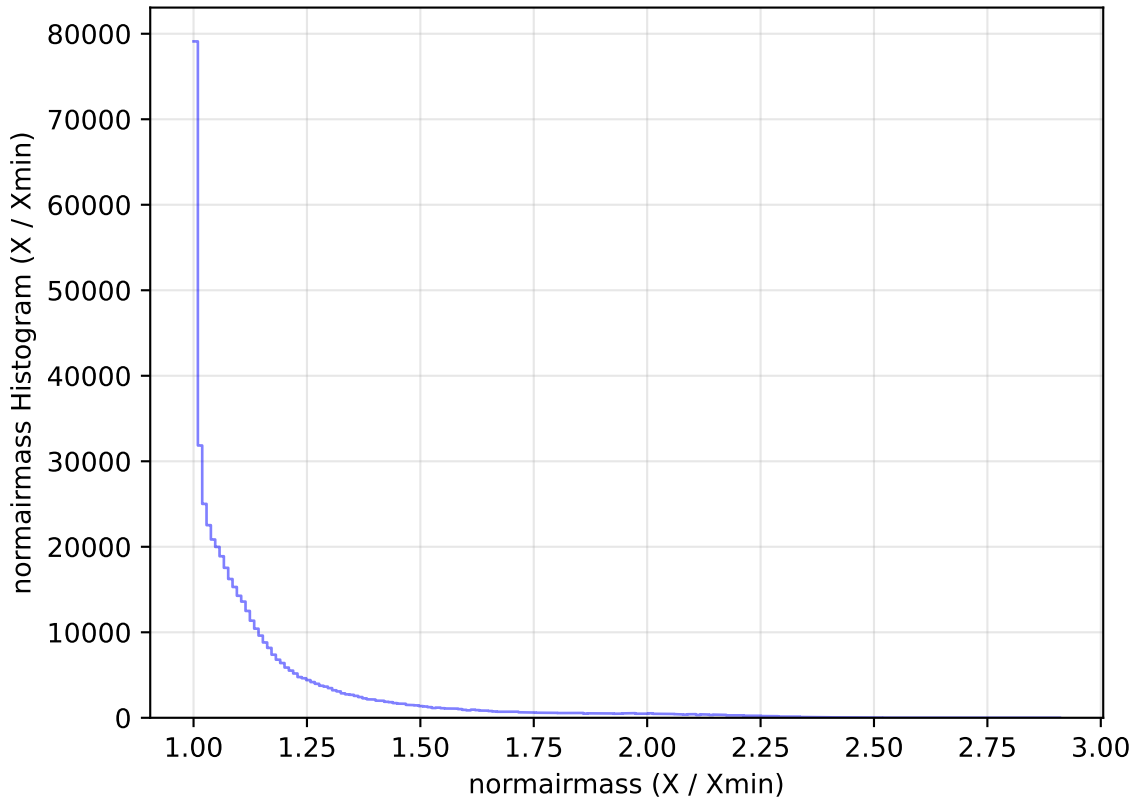
weather_cloudso18v3.4_10yrs All sky r band: normairmass Histogram
