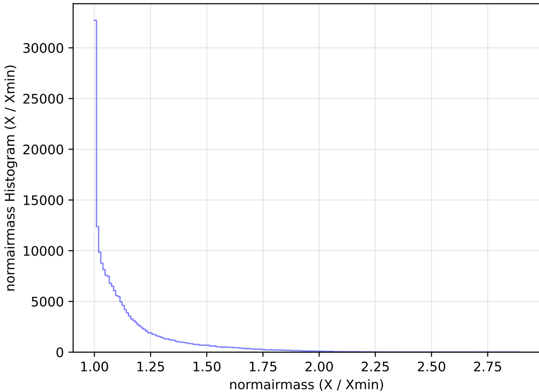
weather_cloudso18v3.4_10yrs All sky g band: normairmass Histogram
