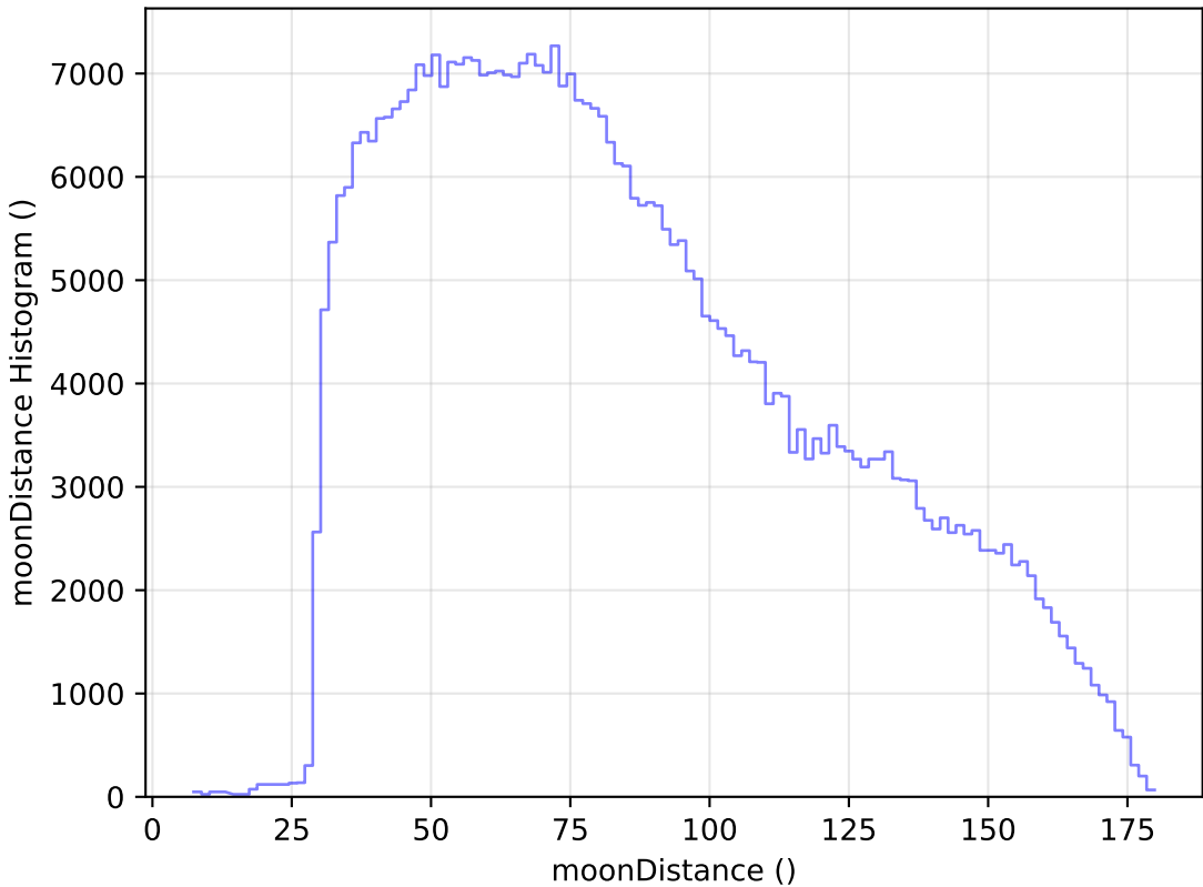
weather_cloudso18v3.4_10yrs WFD z band: moonDistance Histogram
