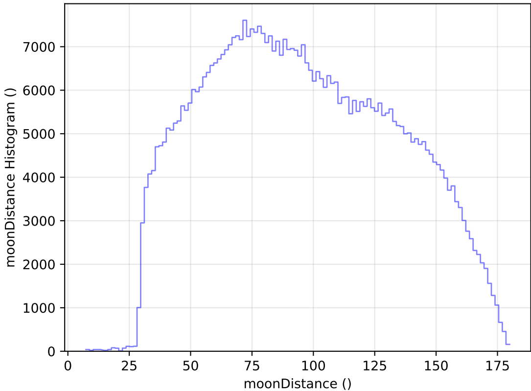
weather_cloudso18v3.4_10yrs WFD i band: moonDistance Histogram
