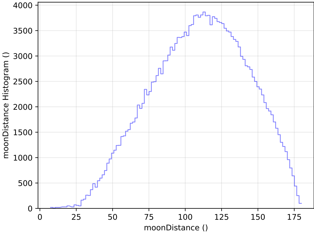
weather_cloudso18v3.4_10yrs WFD g band: moonDistance Histogram
