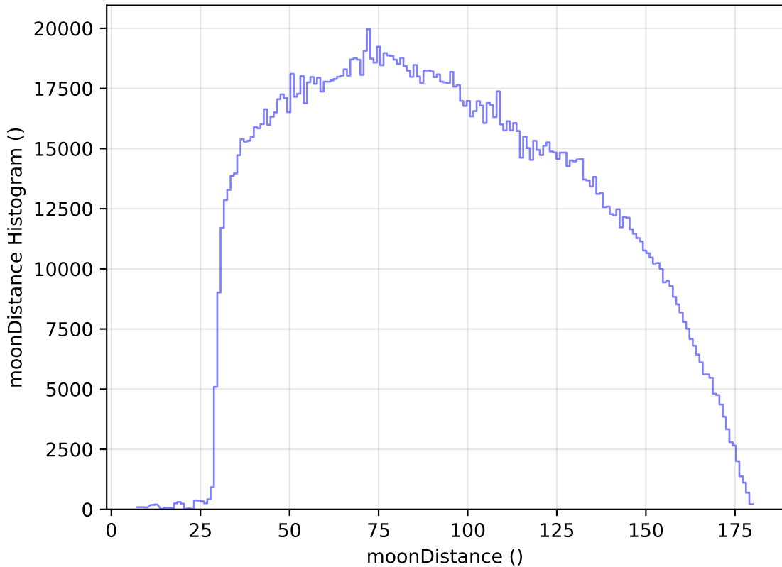
weather_cloudso18v3.4_10yrs WFD all bands: moonDistance Histogram
