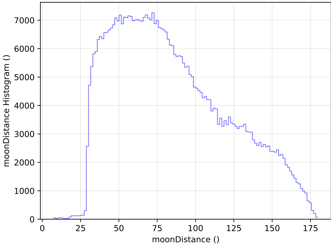
weather_cloudso18v3.4_10yrs All sky z band: moonDistance Histogram
