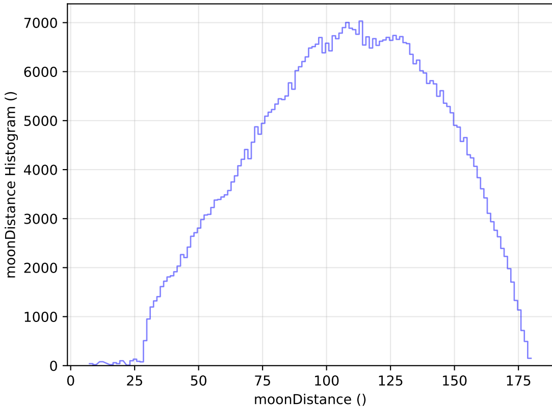
weather_cloudso18v3.4_10yrs All sky r band: moonDistance Histogram
