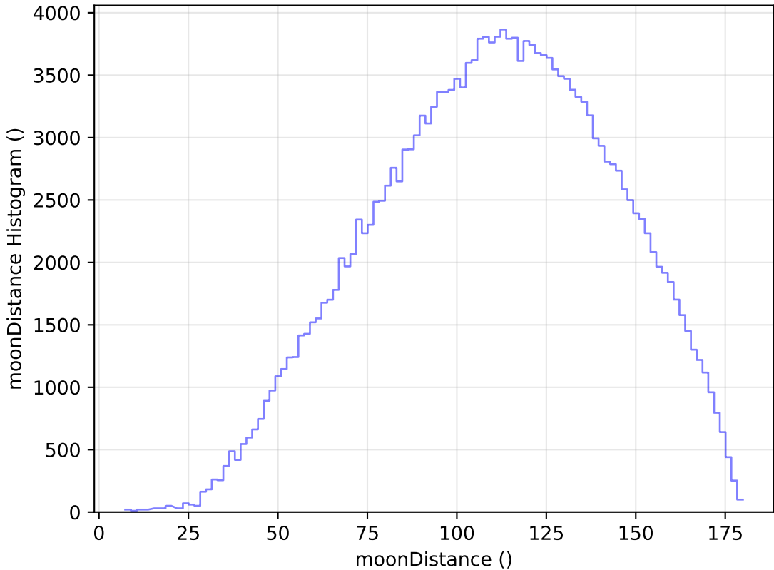
weather_cloudso18v3.4_10yrs All sky g band: moonDistance Histogram
