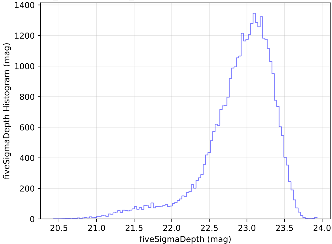
weather_cloudso18v3.4_10yrs Yr 1 z band: fiveSigmaDepth Histogram
