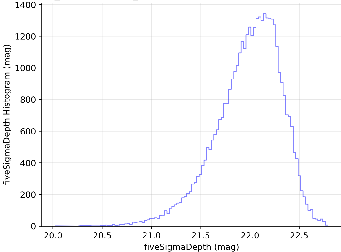
weather_cloudso18v3.4_10yrs Yr 1 y band: fiveSigmaDepth Histogram
