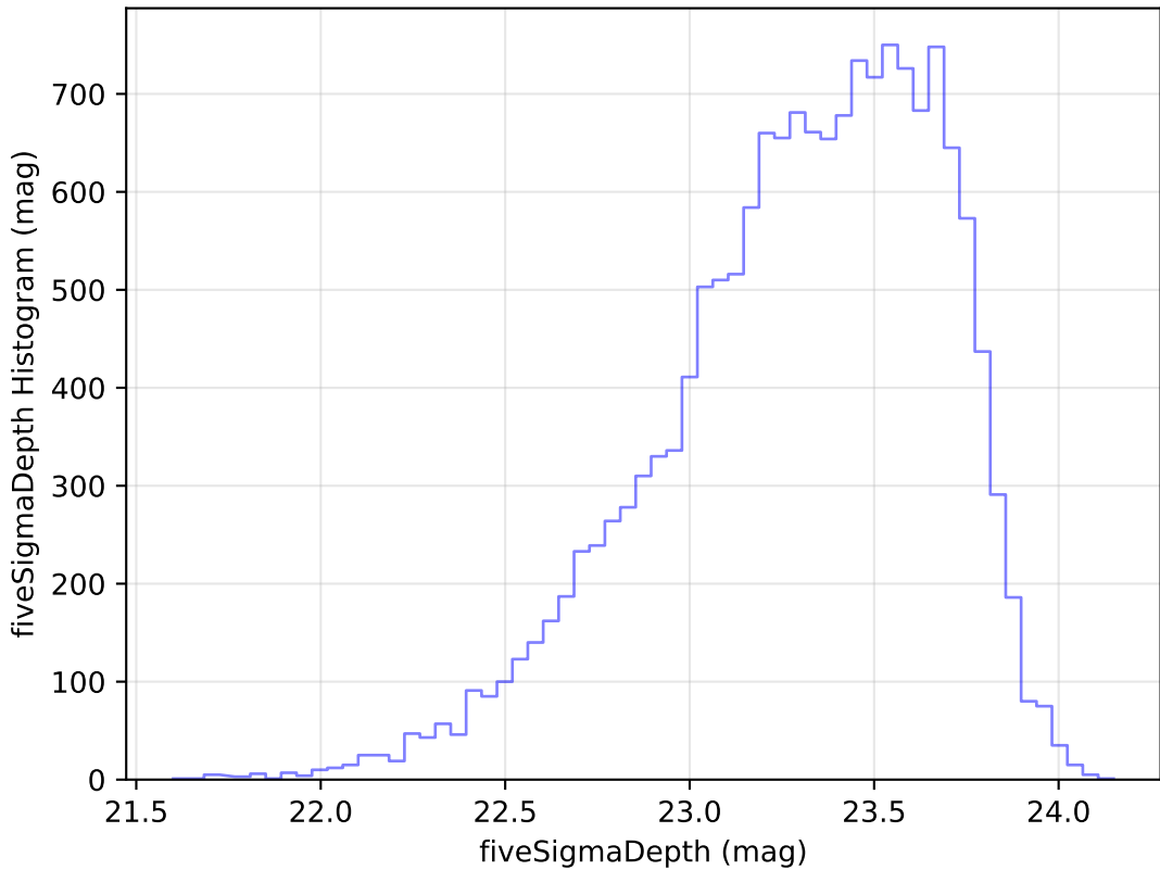
weather_cloudso18v3.4_10yrs Yr 1 u band: fiveSigmaDepth Histogram
