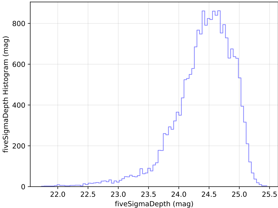
weather_cloudso18v3.4_10yrs Yr 1 g band: fiveSigmaDepth Histogram
