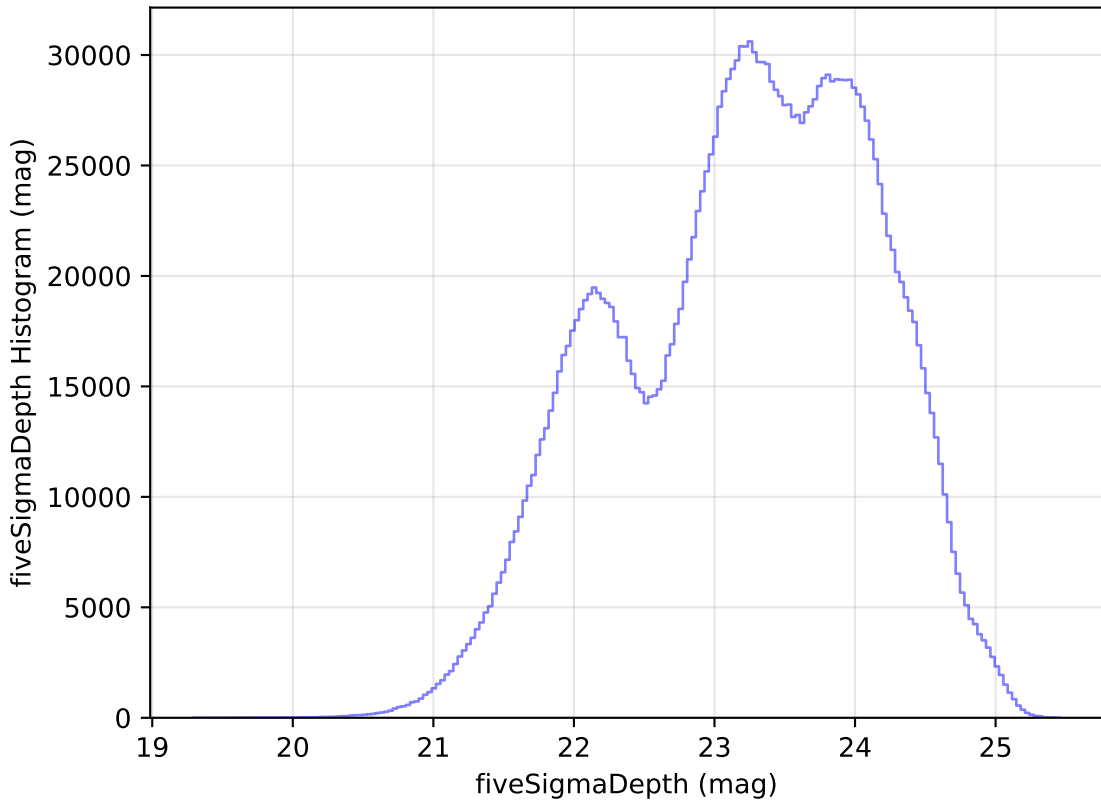
weather_cloudso18v3.4_10yrs WFD all bands: fiveSigmaDepth Histogram
