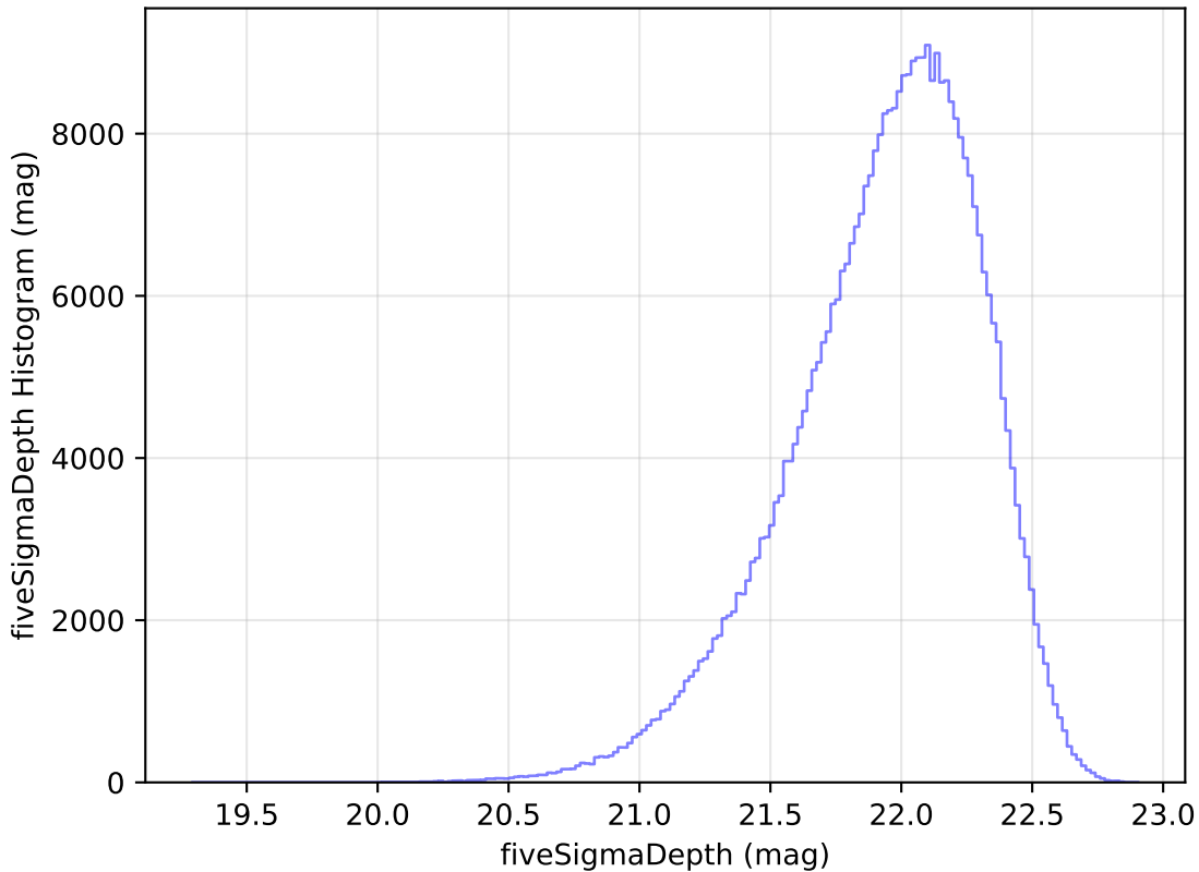
weather_cloudso18v3.4_10yrs All sky y band: fiveSigmaDepth Histogram
