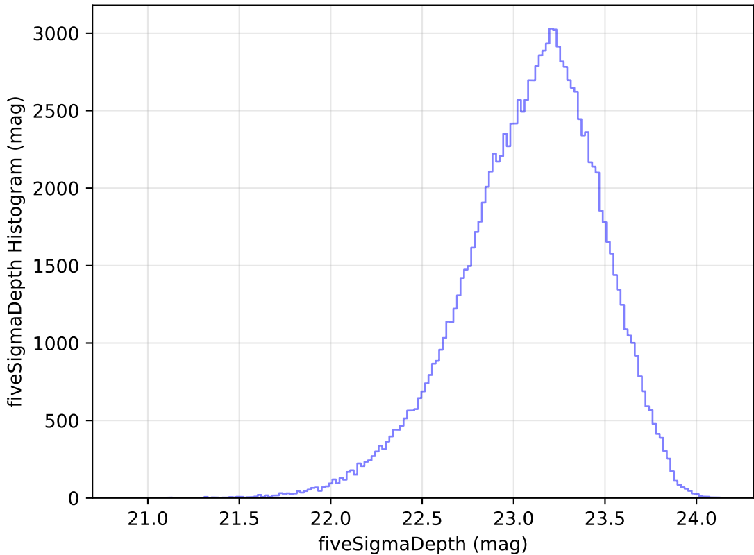
weather_cloudso18v3.4_10yrs All sky u band: fiveSigmaDepth Histogram
