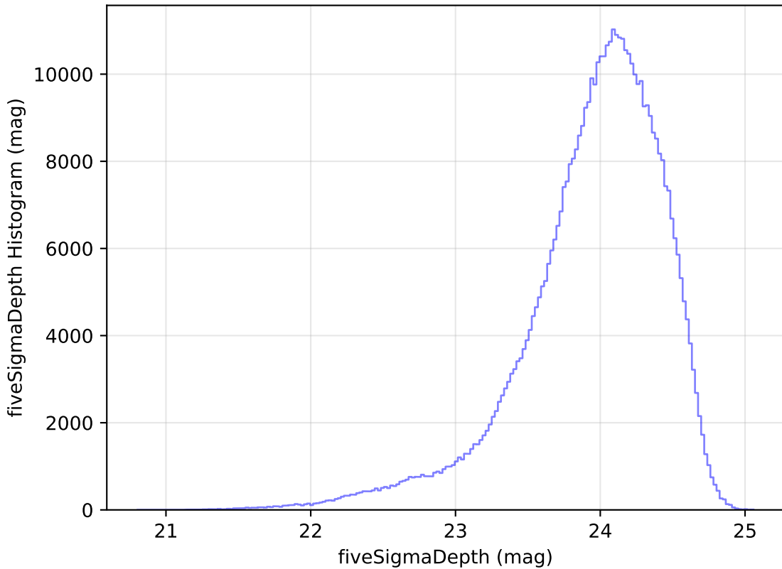
weather_cloudso18v3.4_10yrs All sky r band: fiveSigmaDepth Histogram
