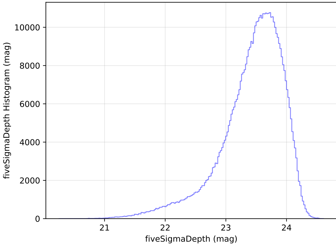
weather_cloudso18v3.4_10yrs All sky i band: fiveSigmaDepth Histogram
