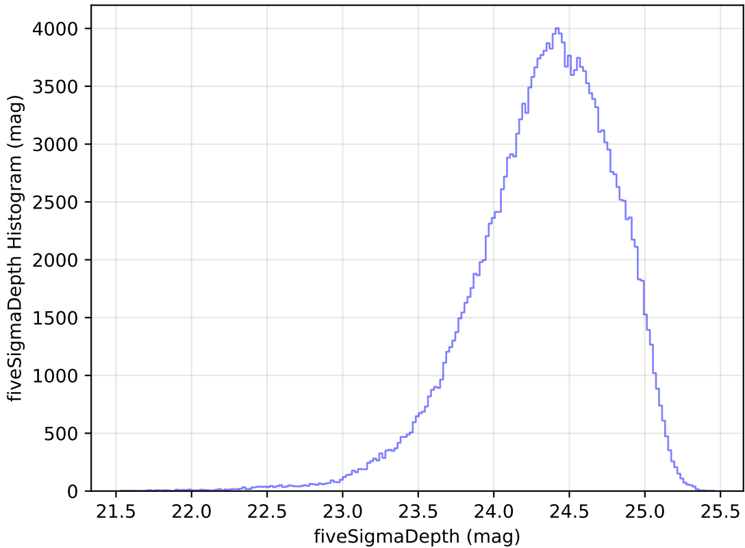
weather_cloudso18v3.4_10yrs All sky g band: fiveSigmaDepth Histogram
