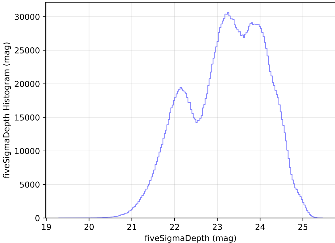
weather_cloudso18v3.4_10yrs All sky all bands: fiveSigmaDepth Histogram
