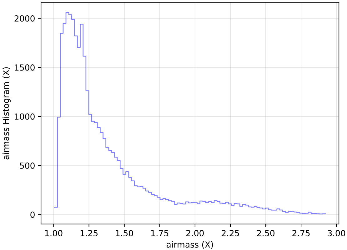
weather_cloudso18v3.4_10yrs Yr 1 z band: airmass Histogram
